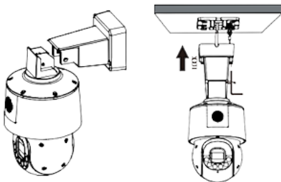
Wall bracket
