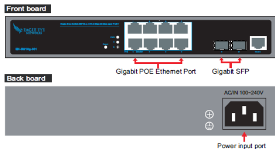
Figure 2: The Board Diagram of an 8 Port 10/100/100 Base-T with a 2 Gigabit RJ45 + 2 Gigabit SFP Switch
