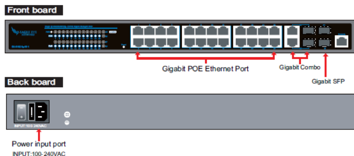
Figure 2: The Board Diagram of a 24 Port 10/100/100 Base-T with a 2 Gigabit RJ45 + 2 Gigabit SFP and 24 PoE Ethernet Switch
