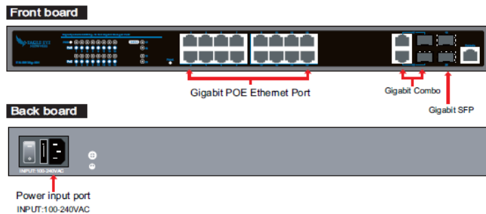
Figure 2: The Board Diagram of an 16 Port 10/100/100 Base-T with a 2 Gigabit RJ45 + 2 Gigabit SFP and 16 PoE Ethernet Switch
